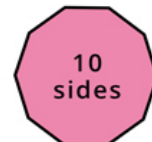
Regular Decagon
